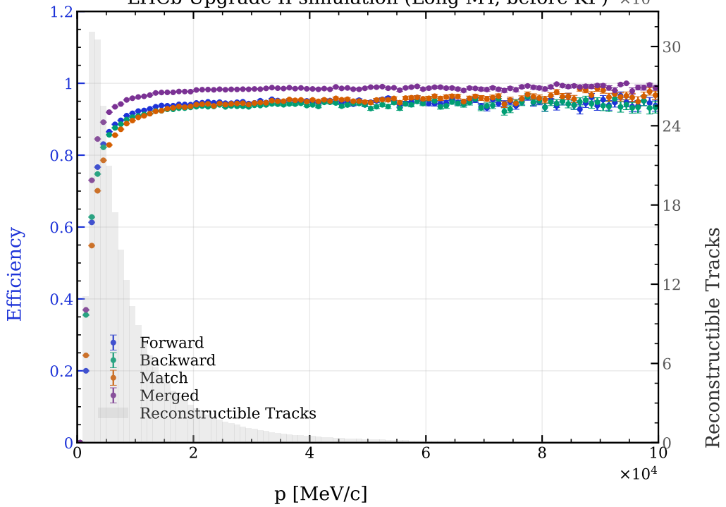
LHCb Upgrade II simulation (Long MT, before KF) \times 10^4
